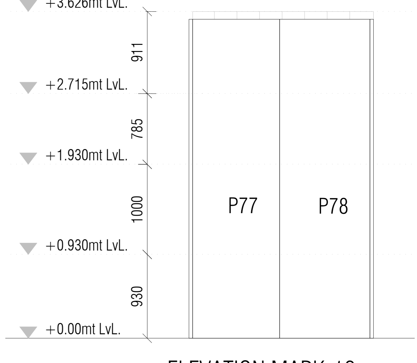
ELEVATION MARK-12 SCALE:- 1:50
