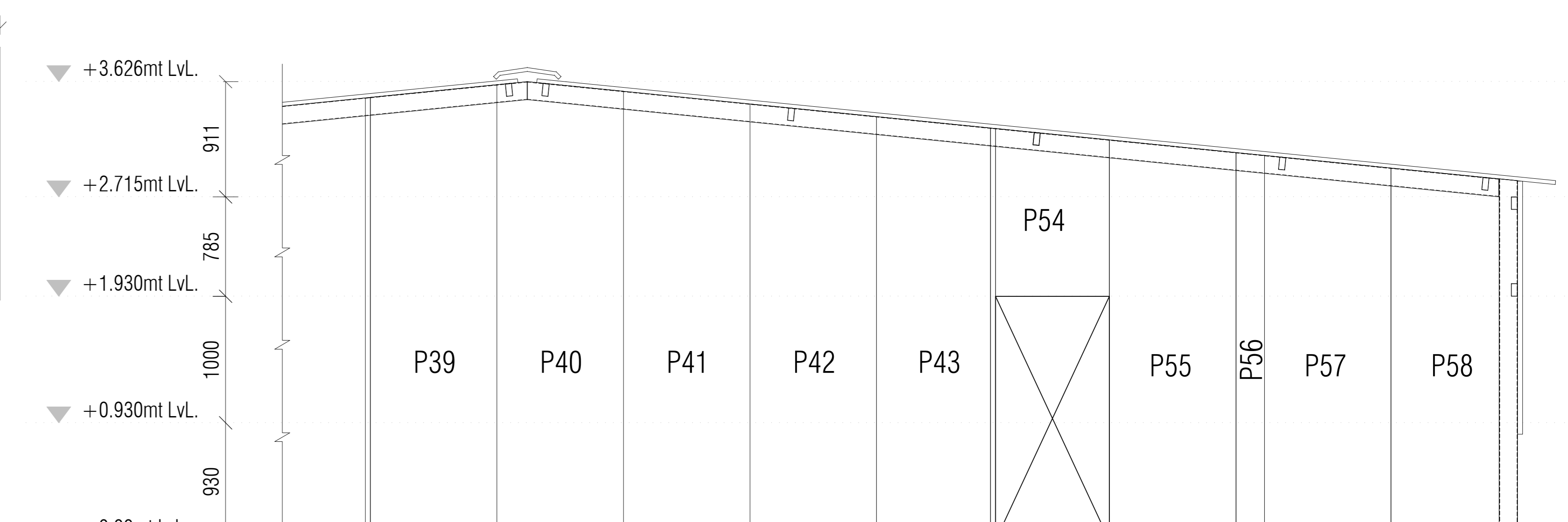
ELEVATION MARK-5 SCALE:- 1:50
