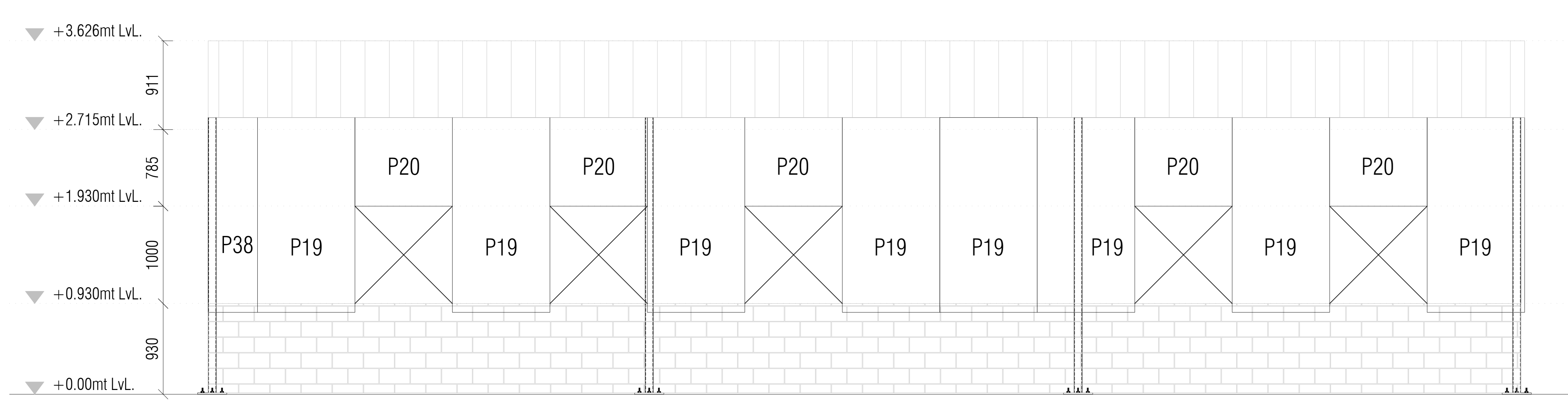
ELEVATION MARK-4 SCALE:- 1:50
