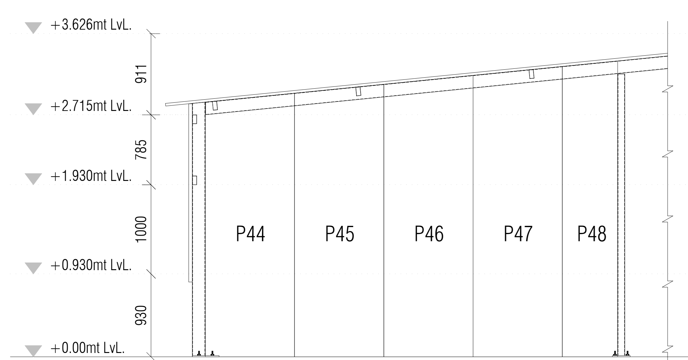
ELEVATION MARK-6 SCALE:- 1:50
