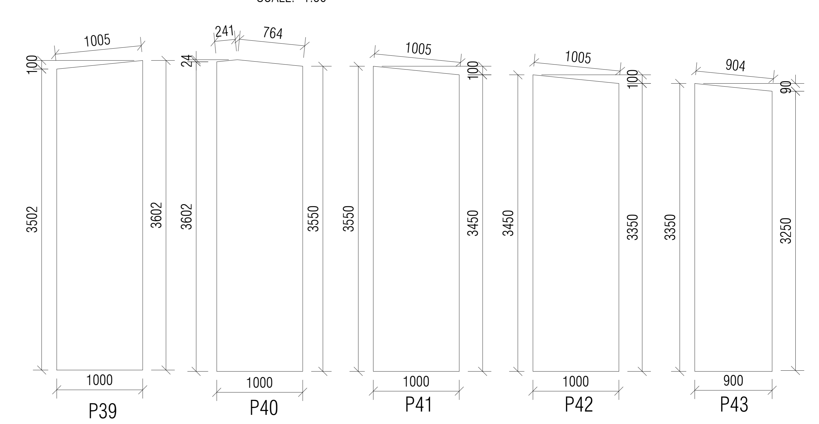
ELEVATION MARK-5 SCALE:- 1:50
