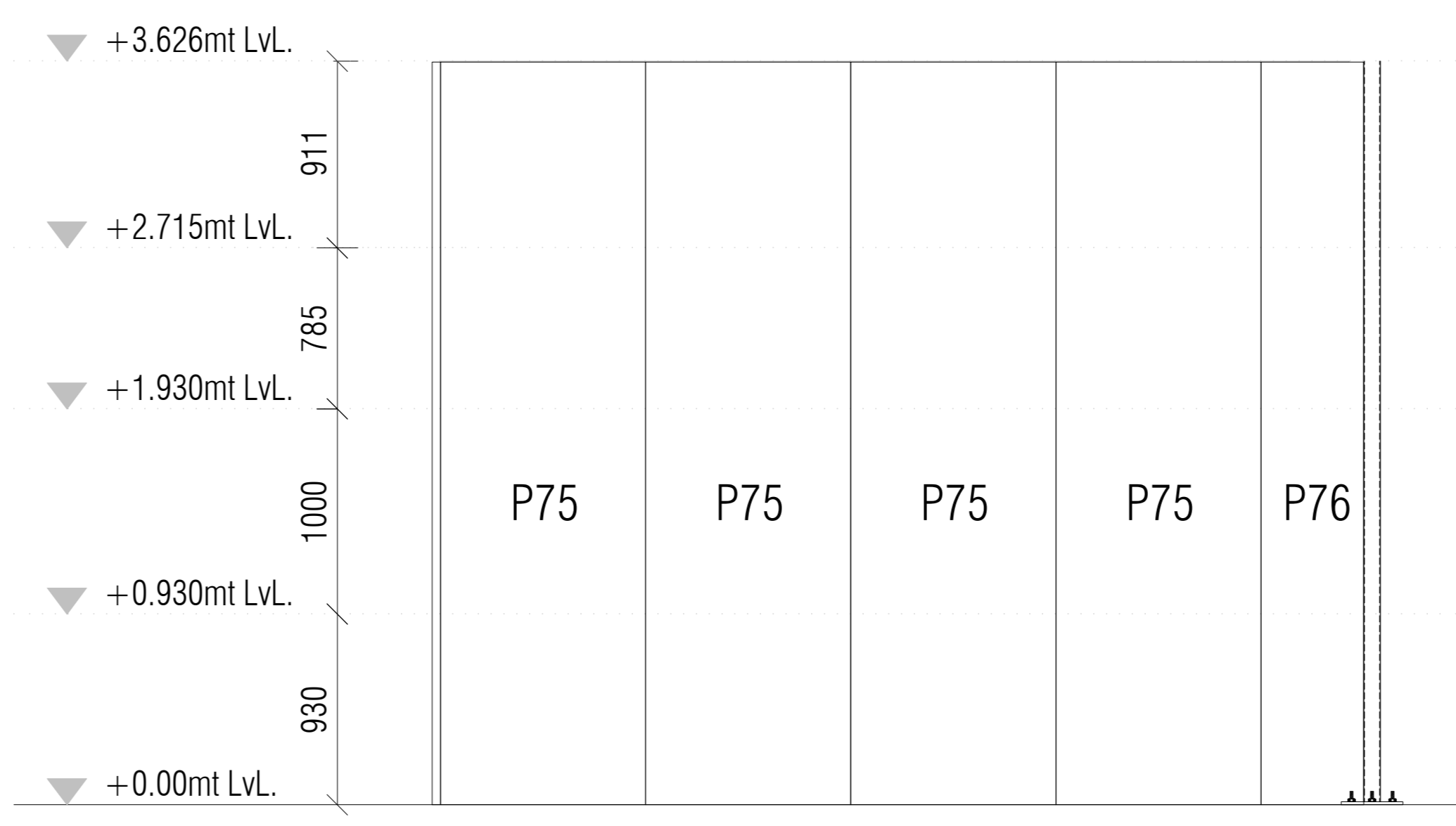
ELEVATION MARK-11 SCALE:- 1:50
