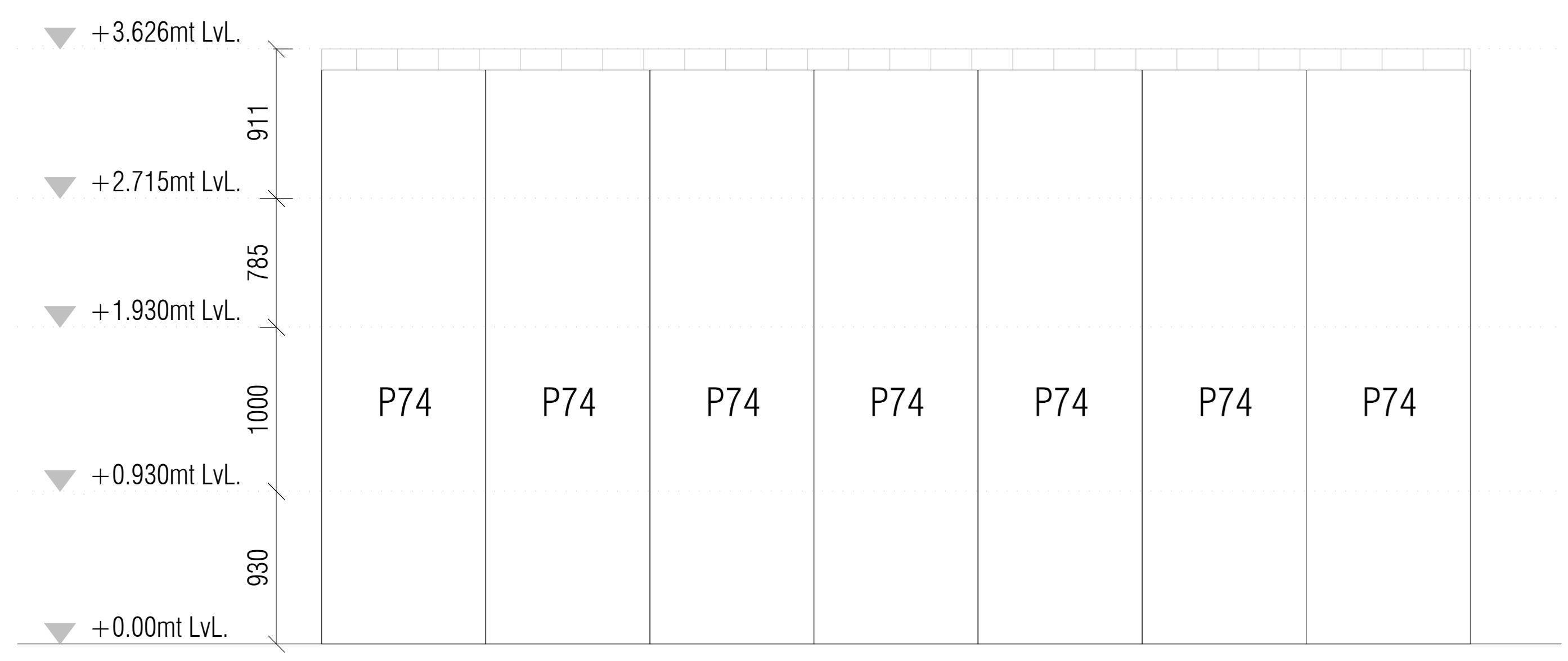
ELEVATION MARK-10 SCALE:- 1:50
