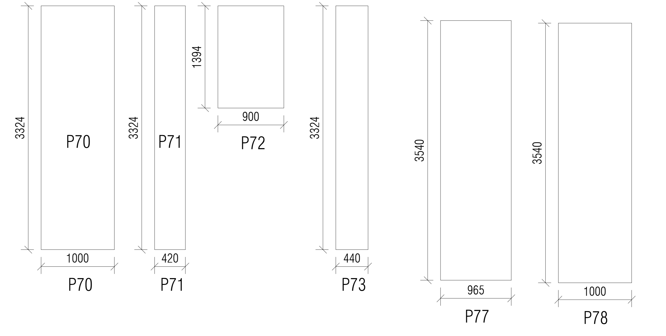
ELEVATION MARK-9 SCALE:- 1:50
