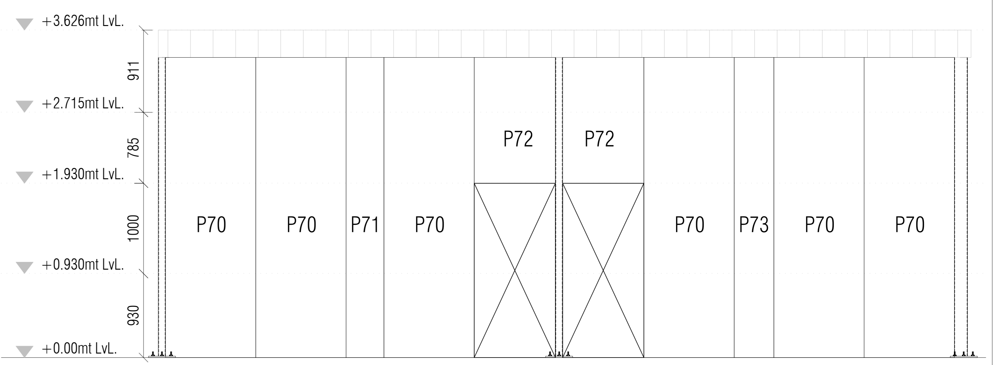
ELEVATION MARK-9 SCALE:- 1:50
