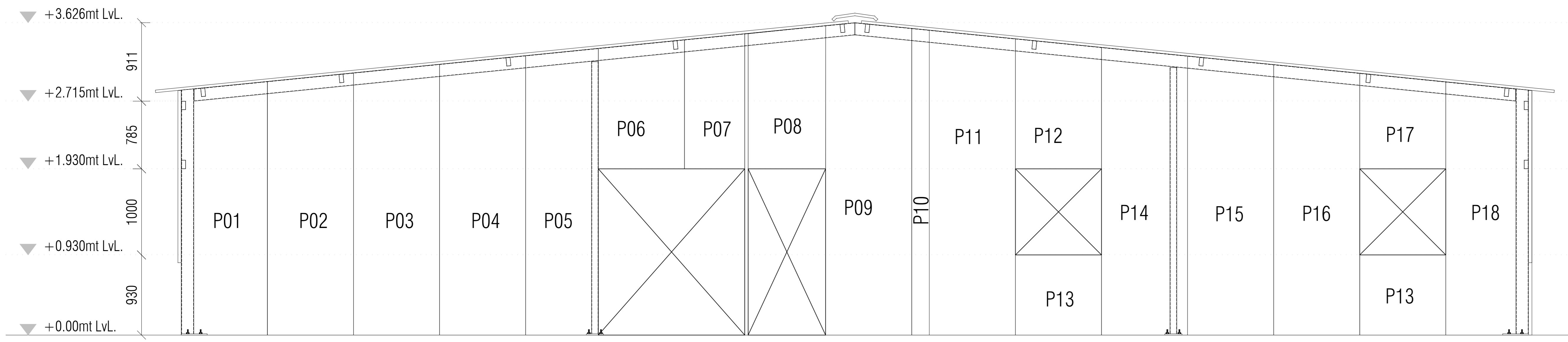
ELEVATION MARK-1 SCALE:- 1:50
