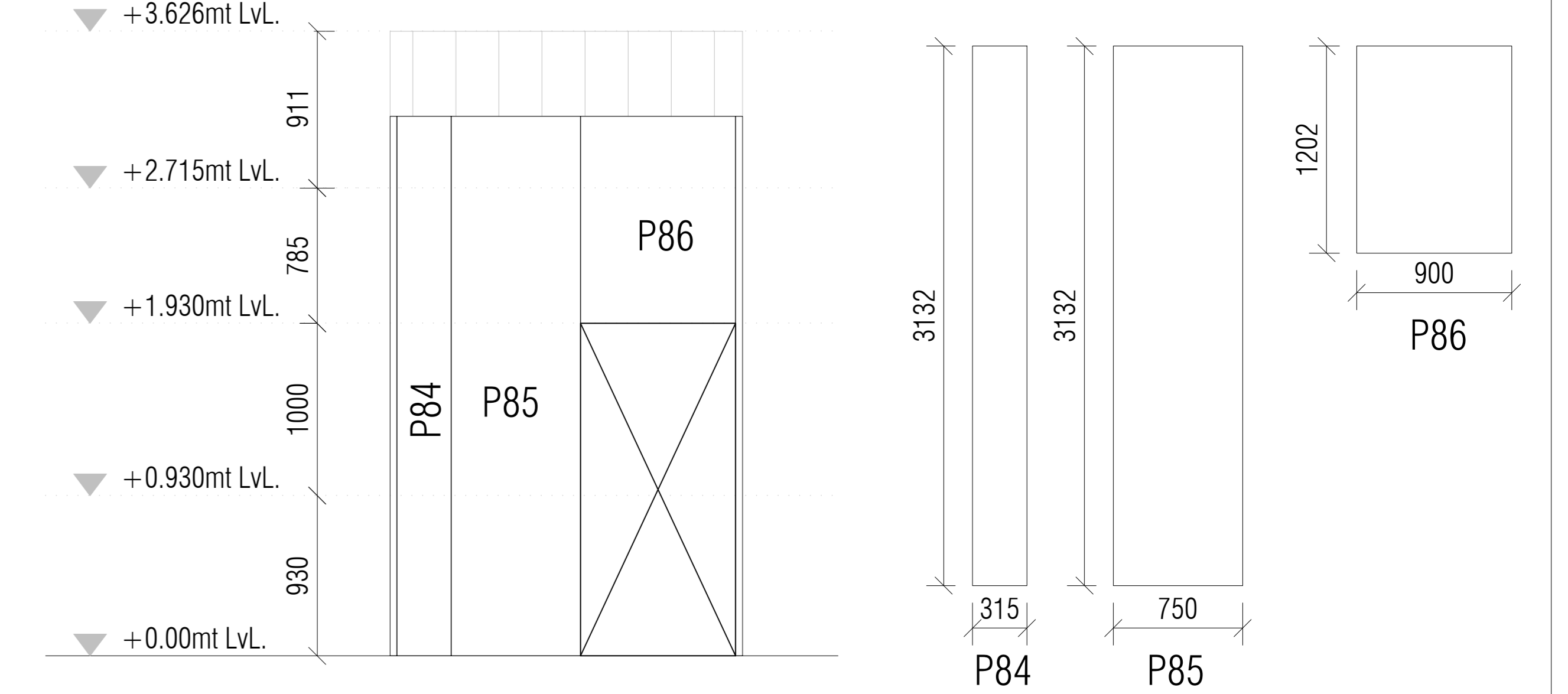
ELEVATION MARK-14 SCALE:- 1:50
