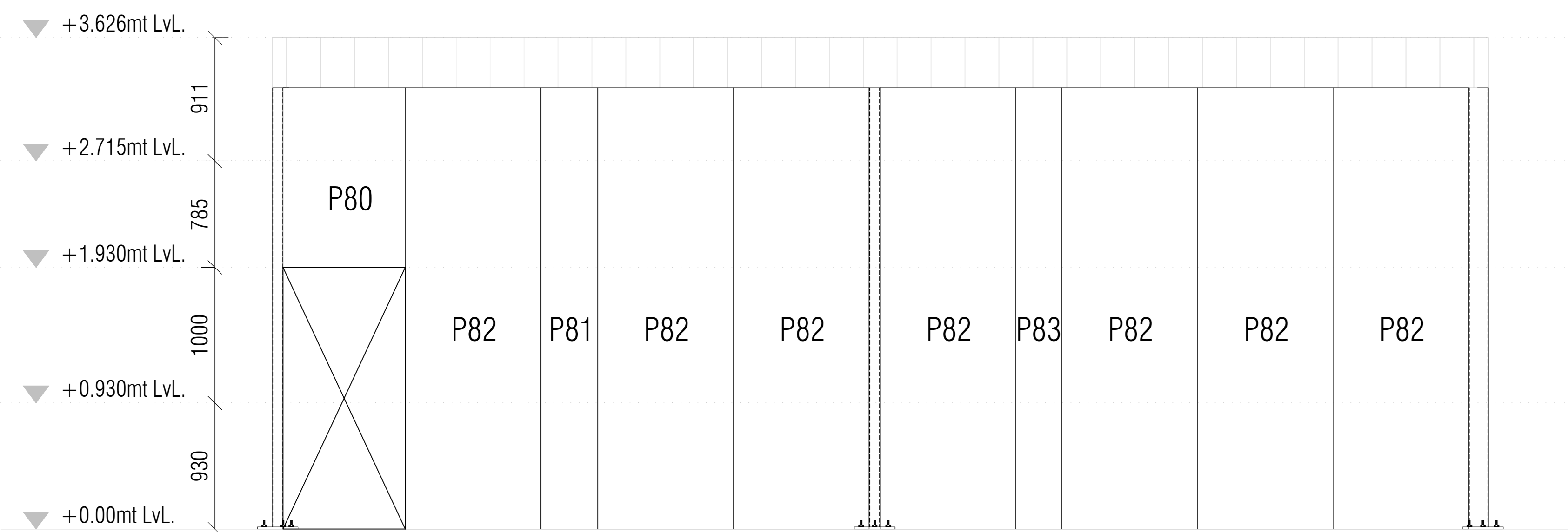
ELEVATION MARK-13 SCALE:- 1:50
